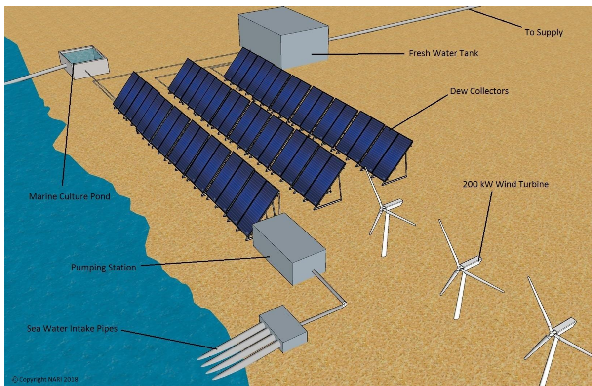
Schematic of Dew Condensation plant
